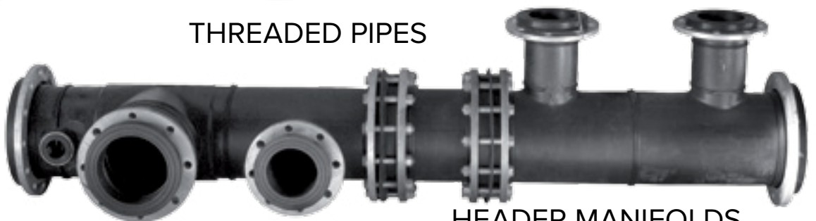
PIPE SPOOLS
