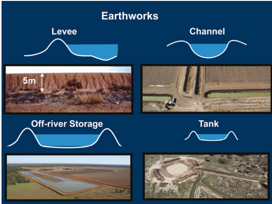
Figure 1: Four examples of flood works: levees, channels, off-river storages and tanks. Other floodplain earthworks can also be used such as flooding and ponding banks, protective earthworks, roads etc.
