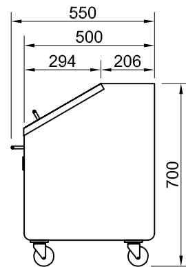
SIDE ELEVATION
