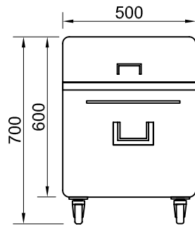
FRONT ELEVATION
