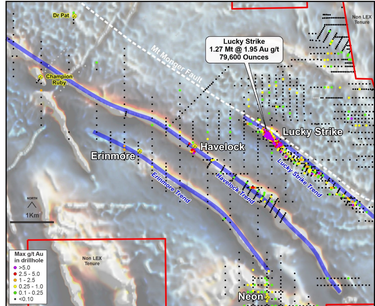
Figure 4: Lucky Strike project area and banded iron formation (BIF) hosted exploration targets
