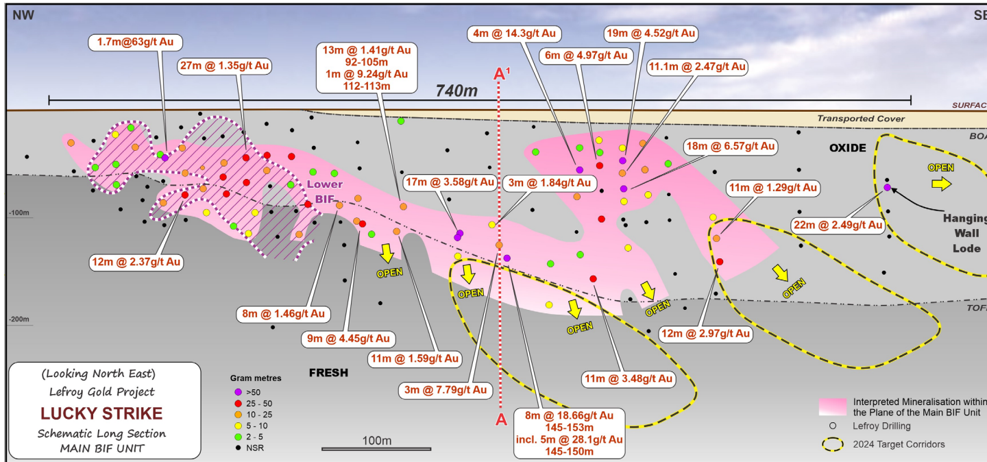
Figure 5: Lucky Strike long section and showing previous LEX intercepts and key drill target corridors.
