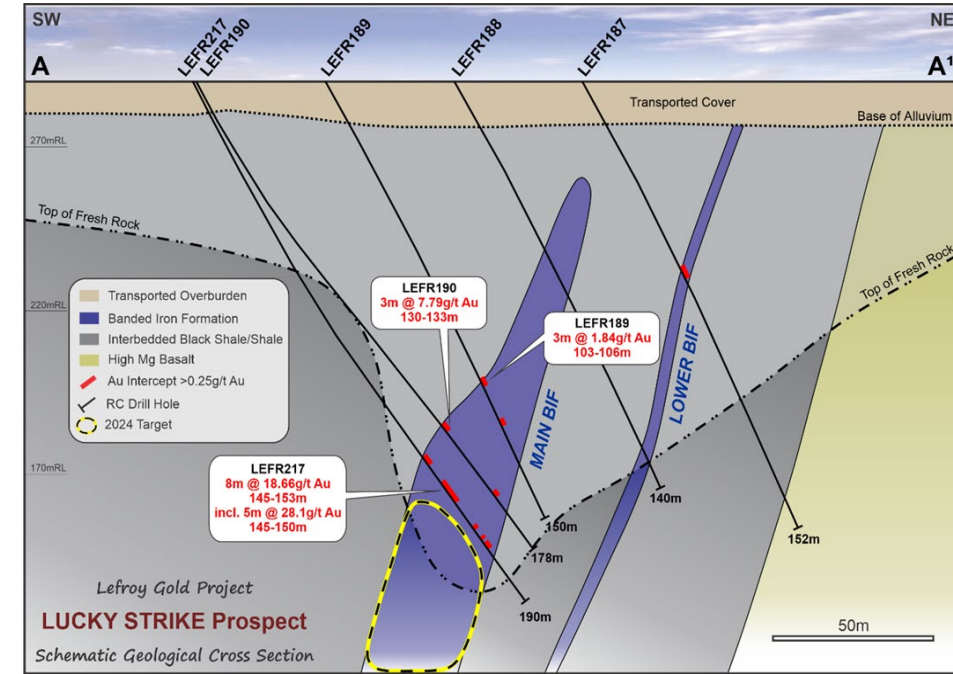
Figure 6: Lucky Strike Cross Section (refer to the section line in Figure 5)
