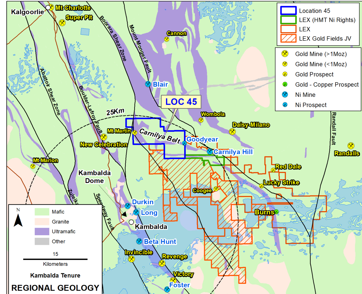
Figure 2: Location of Mt Martin Gold Mine within freehold property, Location 45, in relation to Kalgoorlie, Kambalda and other Lefroy Gold Project assets of the 635km 2 contiguous land package
