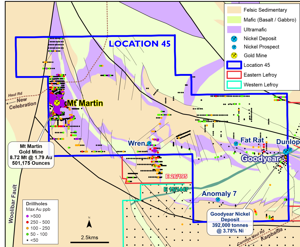
Figure 9: Location 45 Regional exploration upside
