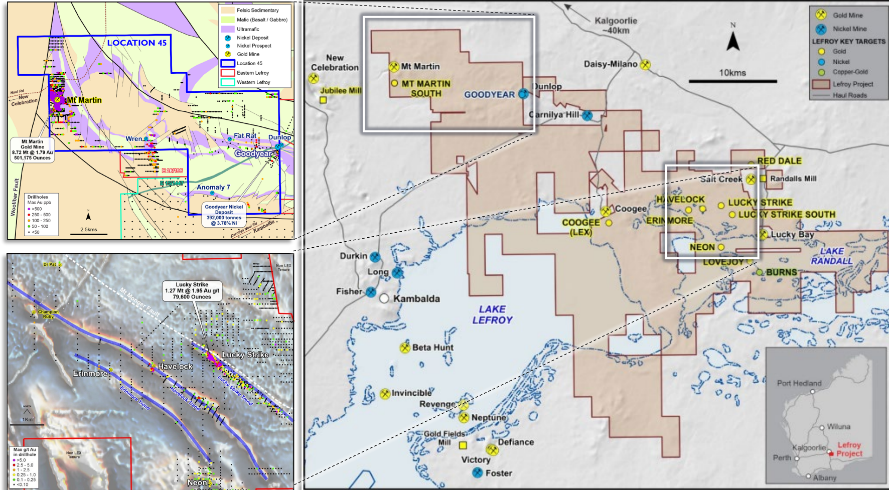
Figure 3: Lefroy tenure and key targets in the Kalgoorlie-Kambalda district
