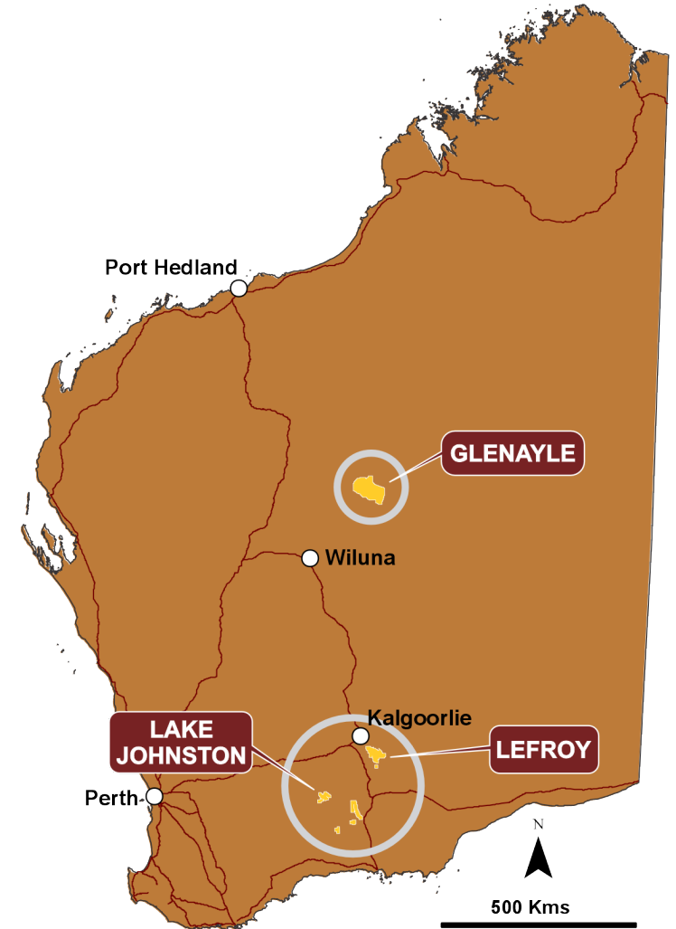
Figure 1: Lefroy's diverse portfolio of high-quality exploration and development assets in Western Australia
