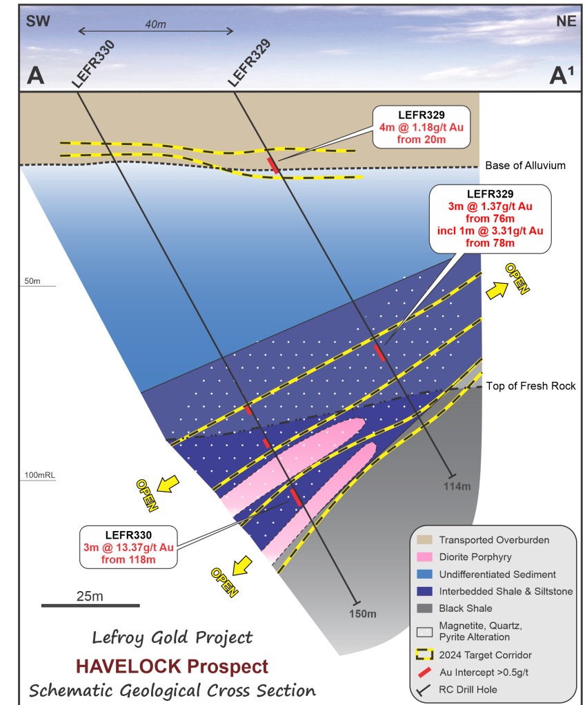
Figure 7: Havelock cross section and exploration upside.
