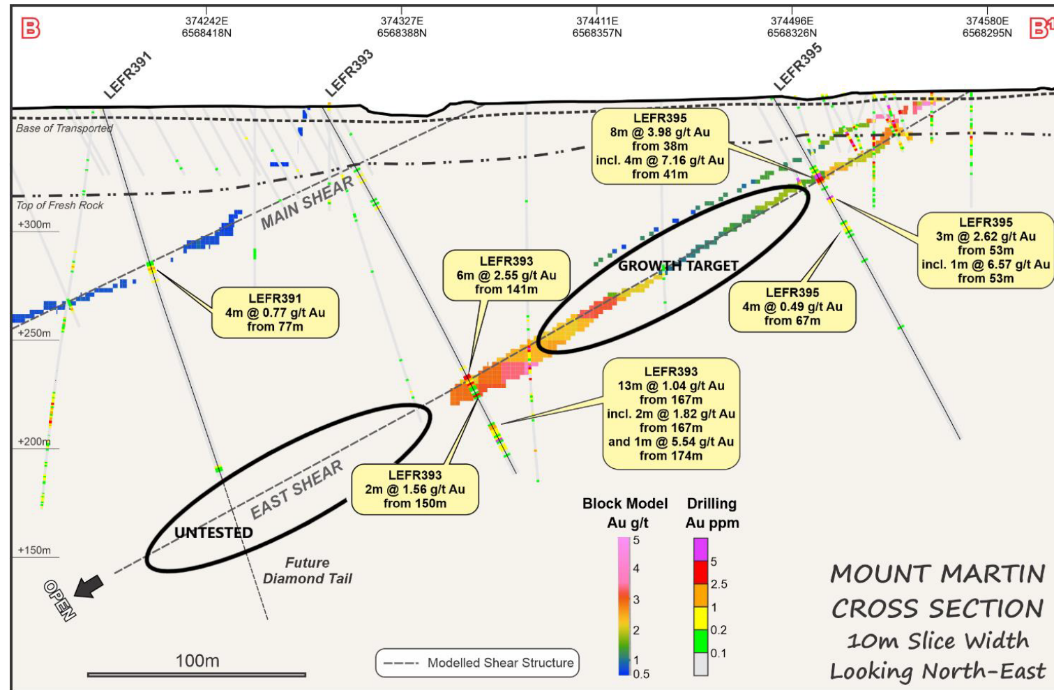
Figure 8: Mt Martin recent RC drilling intersections (January 2024)
