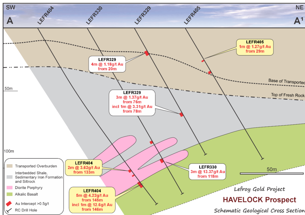
Figure 3: Havelock prospect Section A - A¹ (refer to Figure 2) with recent significant results (yellow boxes).
