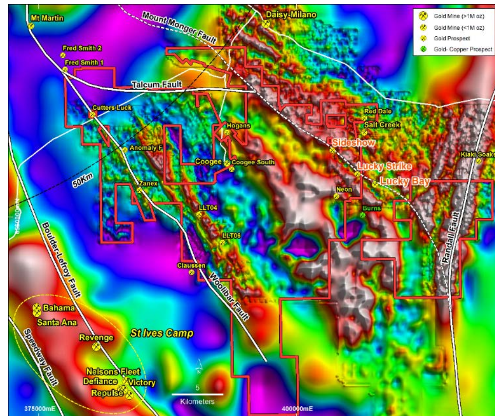
Gravity Bouguer 1VD
