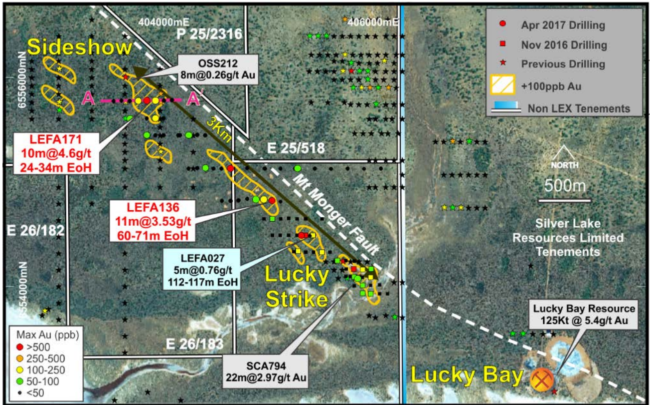
Figure 2 Location of LEX tenements, Lucky Strike Prospect, recent drilling and proximity to the Lucky Bay Open pit. Refer to drill section A-A' in Figure 3.
