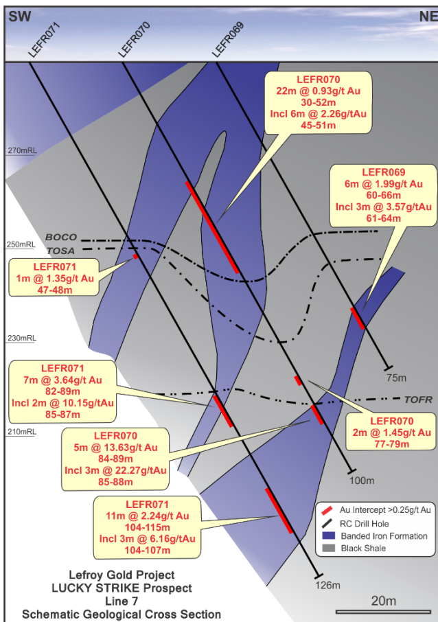
Figure 3 Lucky Strike drill section Line 7
