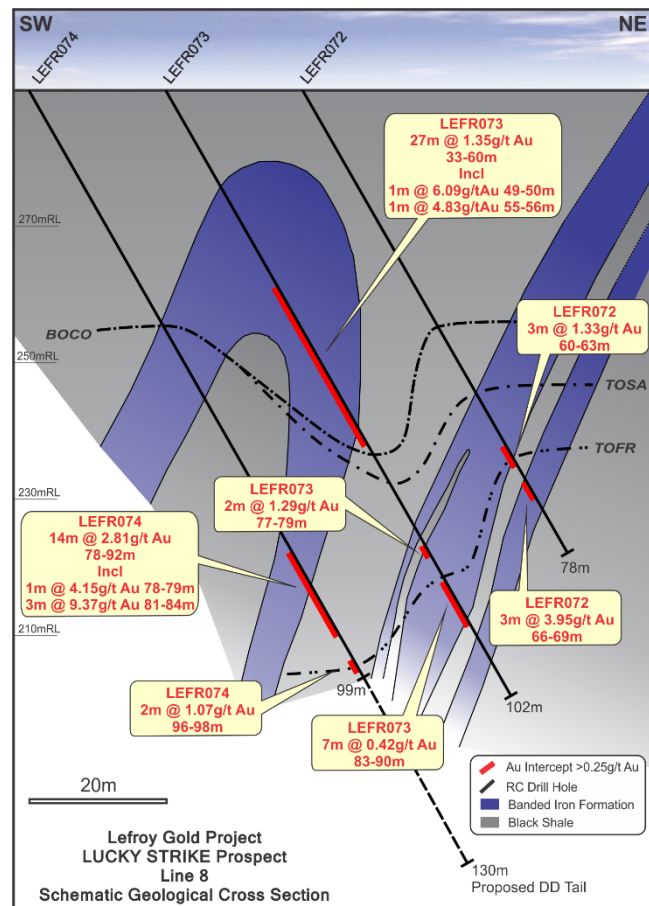
Figure 4 Lucky Strike drill section Line 8
