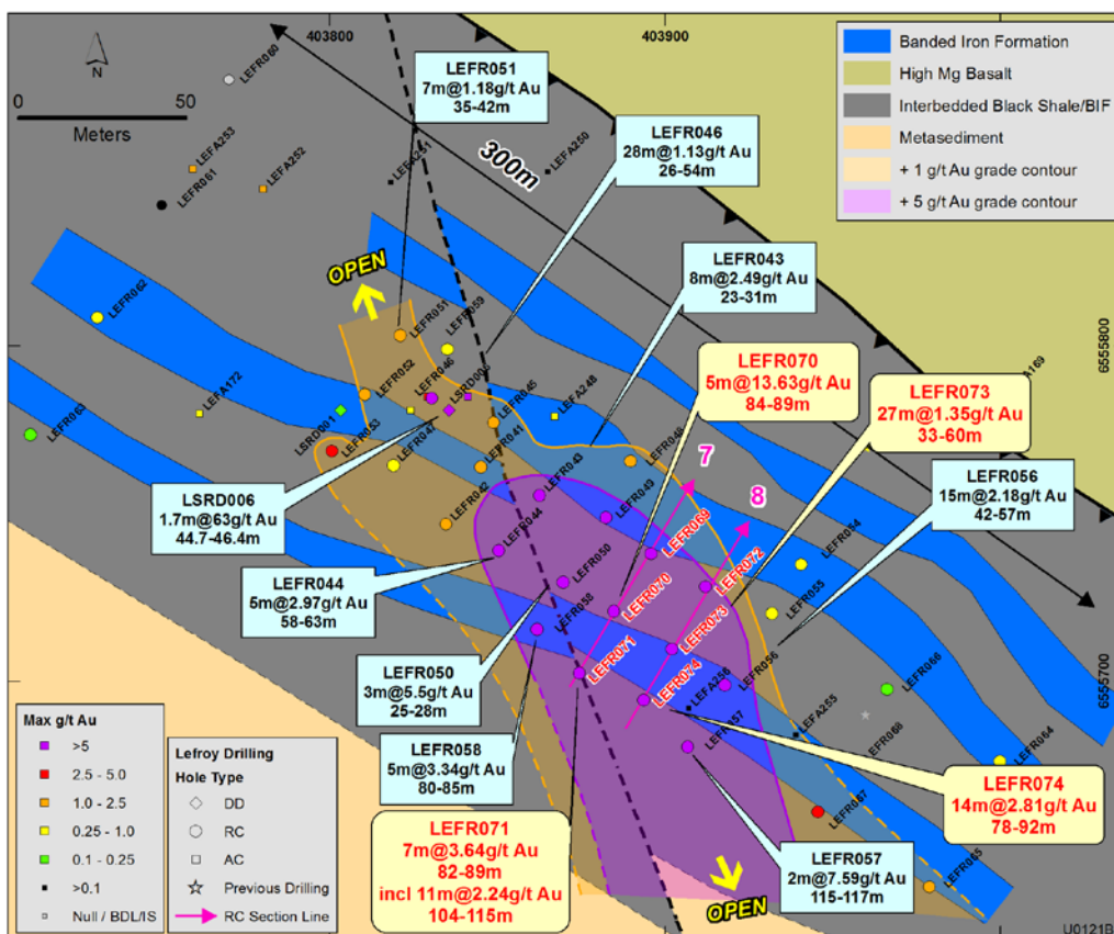
Figure 2 Lucky Strike geology and drill hole plan highlighting key recent (sections 7&8) and earlier drill intersections. (Refer Figures 4 & 5 for drill sections for Lines 7 and 8)
