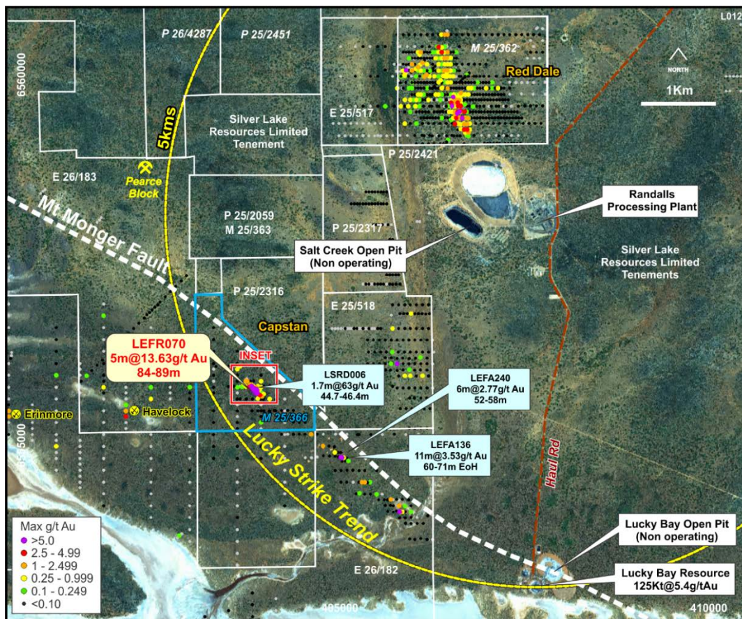
Figure 1 Location of the Lucky Strike Trend relative to the Red Dale and Capstan Prospects and proximity to the Randalls Processing Facility (SLR). The key Lucky Strike Trend gold intersections are also highlighted (refer to Figure 2 for detailed inset map and recent drilling). The Mining Lease application is highlighted in blue.
