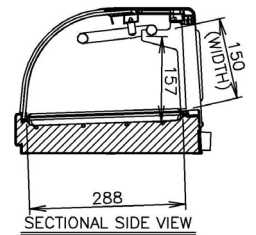
SECTIONAL SIDE VIEW
