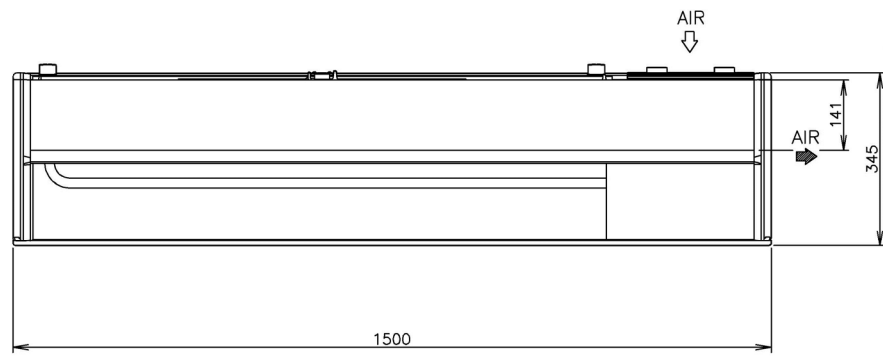
VIEW A (REAR)
