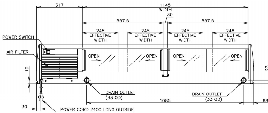
VIEW A (REAR)
