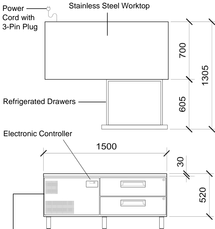
Side Mounted Integral Refrigeration Unit
