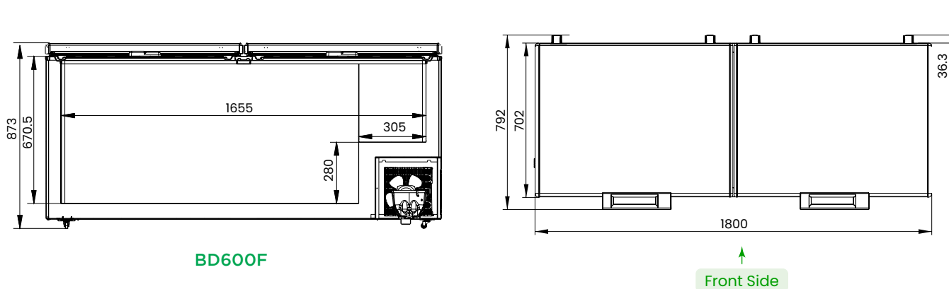
↑ Front Side
