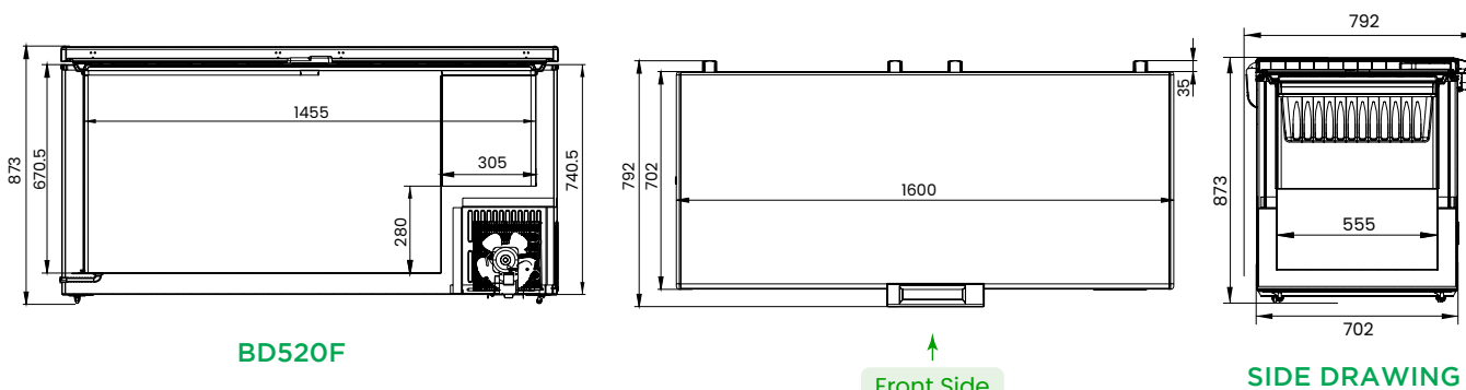
↑ Front Side
