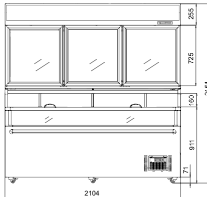
210 combined freezer
